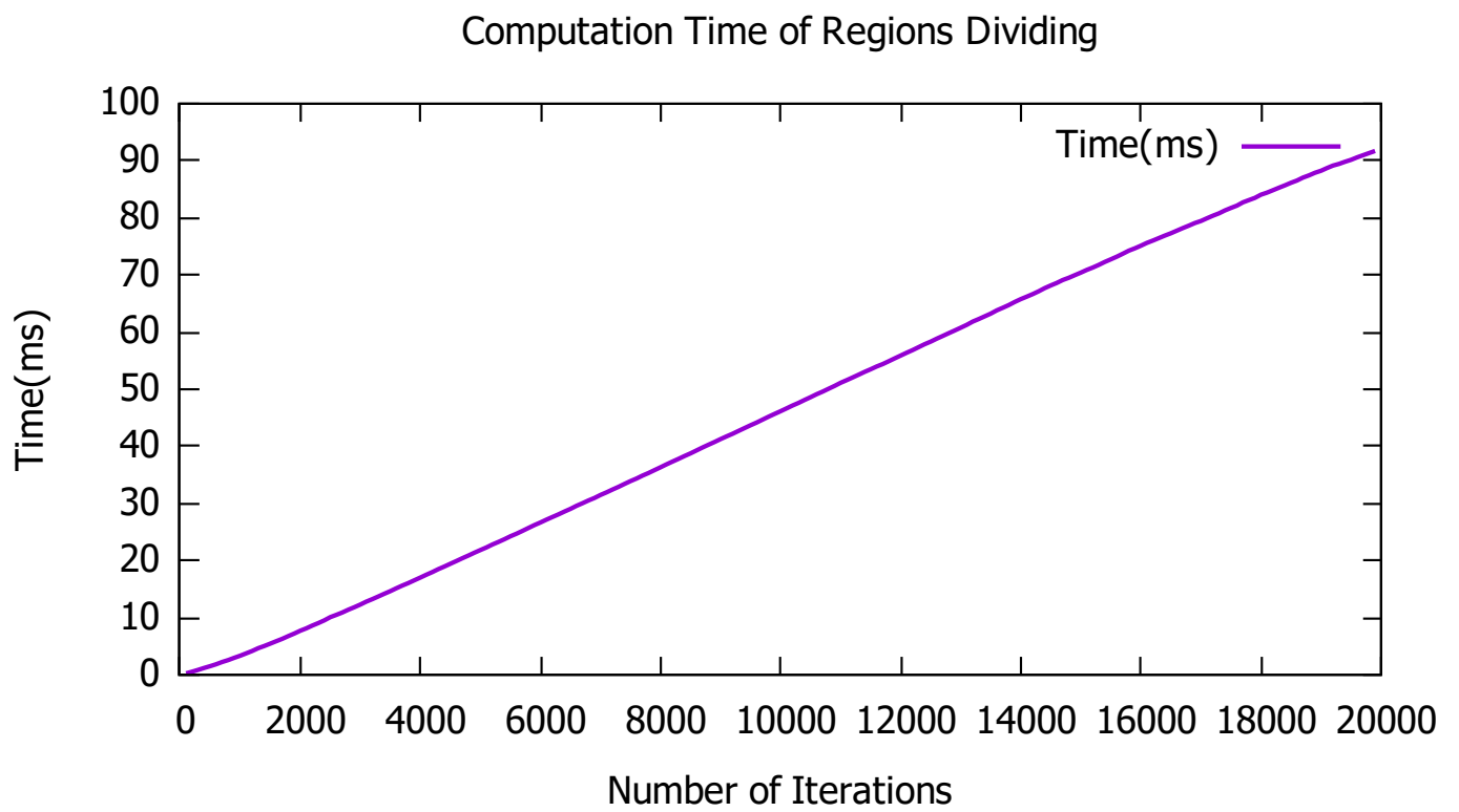
Fig. 10. Computation Time of Regions Dividing
