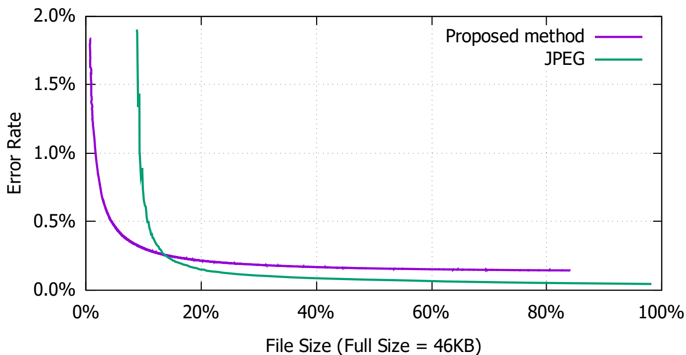
Fig. 9. Proposed method and JPEG comparing
