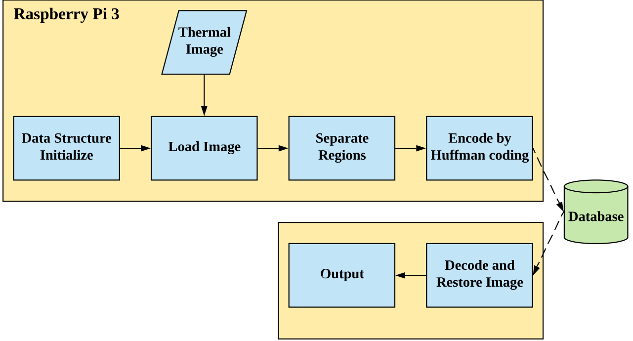
Fig. 4. System Architecture
