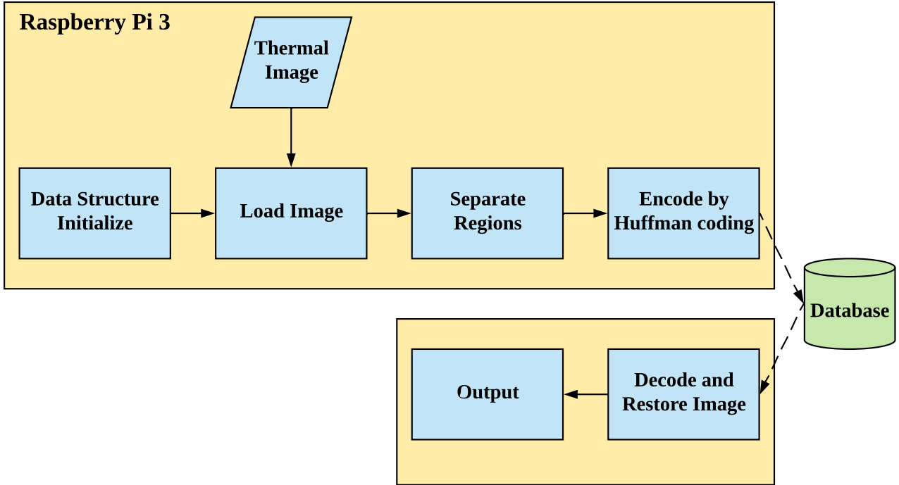
Fig. 4. System Architecture
