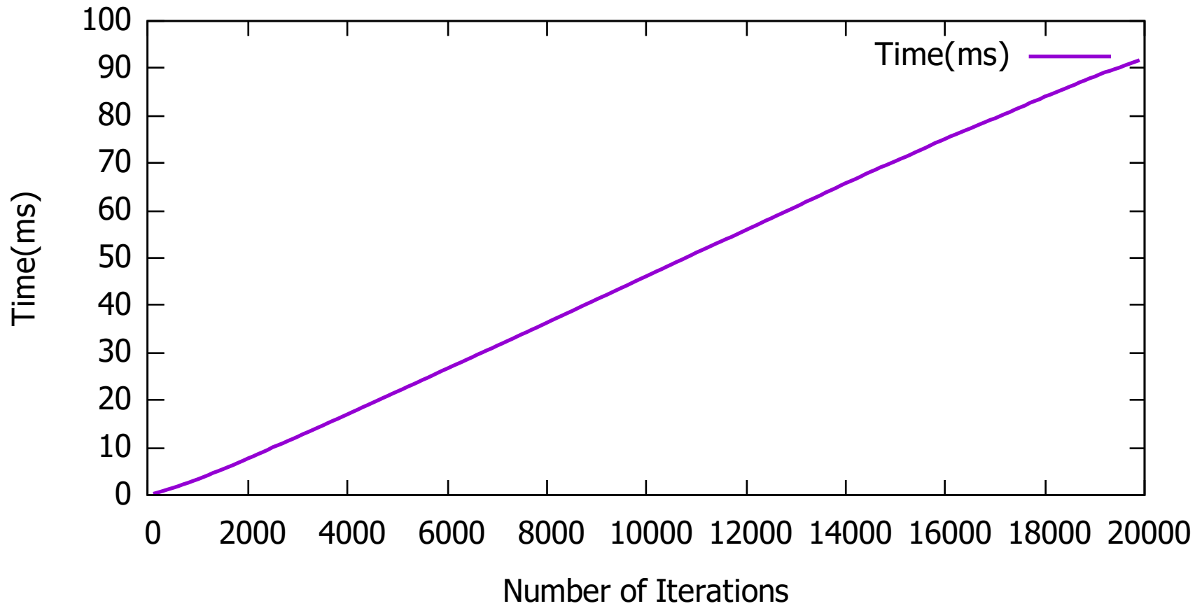
Computation Time of Regions Dividing
